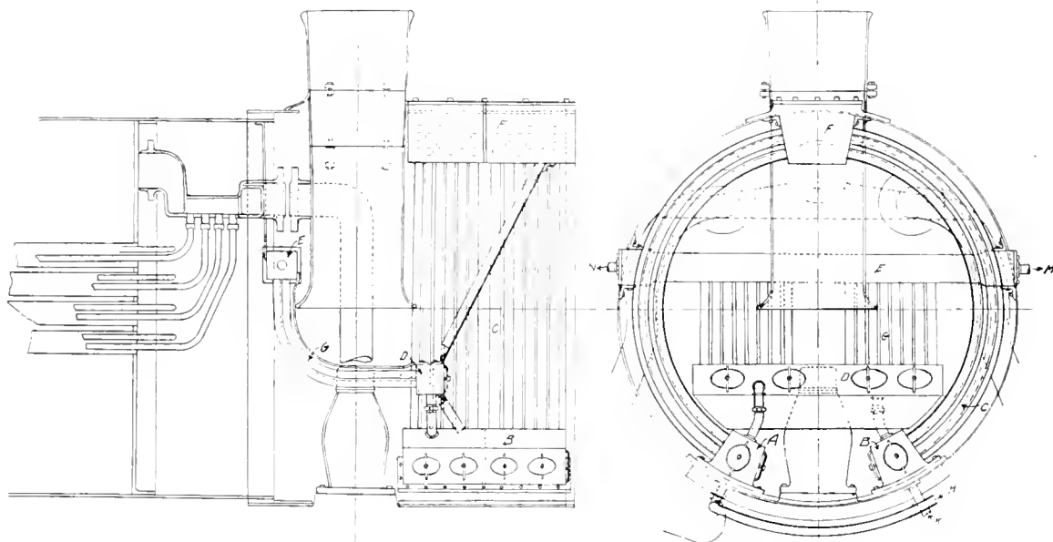
A, B, D, E and F are cast steel headers. C and G are 2-in. steel tubes headed and welded to the headers.
